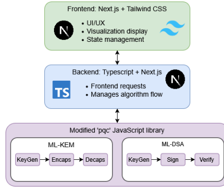
Fig. 11: Architecture of Latviz's ML-KEM and ML-DSA visualization
