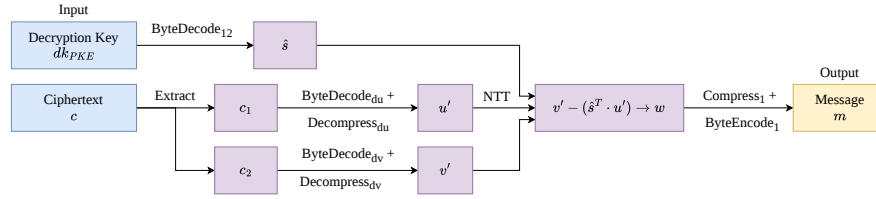
Fig. 6: Kyber Decryption Algorithm K-PKE.Decrypt
