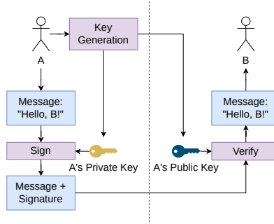
Fig. 7: Simplified digital signature scheme
