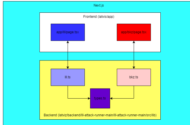
Fig. 12: Program structure of Latviz's LLL and BKZ visualization
