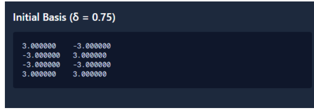
Fig. 13: The initial basis panel (LLL)
