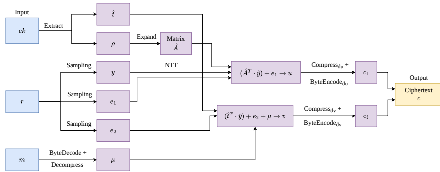
Fig. 5: Kyber Encryption Algorithm K-PKE.Encrypt
