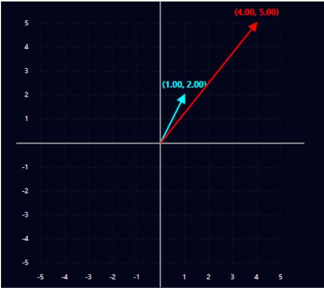
Fig. 16: Basis vectors from the input matrix, represented in the Cartesian coordinate within a Euclidean space
