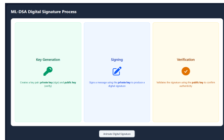
Fig. 18: ML-DSA Process
