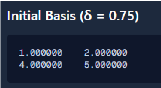
Fig. 15: Basis vectors from the input matrix
