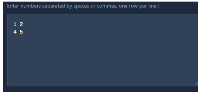
Fig. 14: The input matrix
