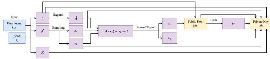
Fig. 8: ML-DSA Internal Keygen Algorithm ML-DSA.KeyGen_internal
