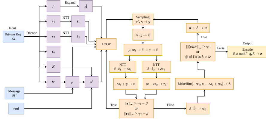
Fig. 9: ML-DSA Internal Signing Algorithm ML-DSA.Sign_internal
