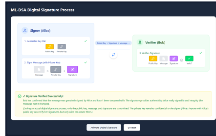
Fig. 19: ML-DSA Process Animation
