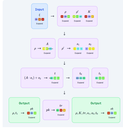
Fig. 28: ML-DSA Full Animation Section (Step 9)
